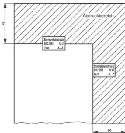
ChronoDater 920/922/925
